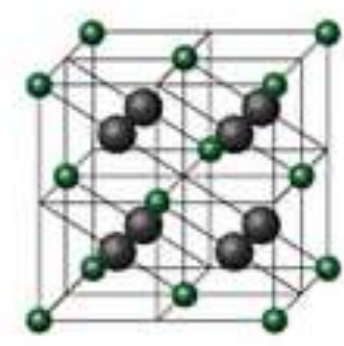
CaF 2
